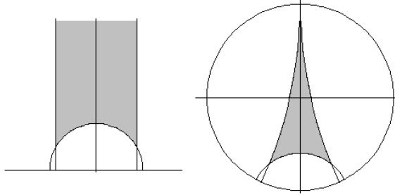
Figure 1. (Left) A fundamental region in the upper half-plane for \left\langle \begin{pmatrix} 1 & \sqrt{3} \\ 0 & 1 \end{pmatrix}, \begin{pmatrix} 0 & -1 \\ 1 & 0 \end{pmatrix} \right\rangle , corresponding to the case p = 6 . Here \mathcal{R} = \left\{z \in \mathbb{C} : |z| > 1, \operatorname{Re} z < \frac{\sqrt{3}}{2}, \operatorname{Im} z > 0\right\} . (Right) The same hyperbolic triangle represented in the Poincaré disc, via the conformal map z \mapsto i \left(\frac{z - 4i}{z + 4i}\right) .
