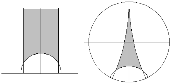
Figure 1. ( Left ) A fundamental region in the upper half-plane for \left\langle \begin{pmatrix} 1 & \sqrt{3} \\ 0 & 1 \end{pmatrix}, \begin{pmatrix} 0 & -1 \\ 1 & 0 \end{pmatrix} \right\rangle , corresponding to the case p = 6 . Here \mathcal{R} = \left\{z \in \mathbb{C} : |z| > 1, \operatorname{Re} z < \frac{\sqrt{3}}{2}, \operatorname{Im} z > 0\right\} . ( Right ) The same hyperbolic triangle represented in the Poincaré disc, via the conformal map z \mapsto i \left(\frac{z - 4i}{z + 4i}\right) .
